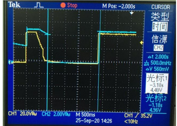
Output response & load (5V / 1.2A)
